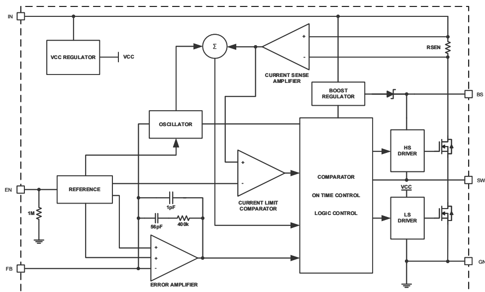
Block Diagram
