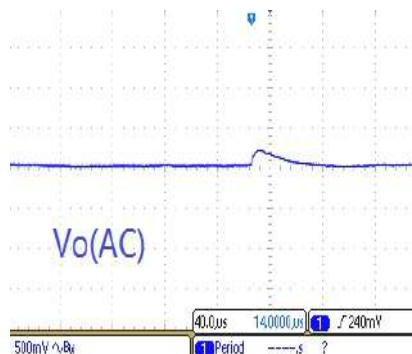
Fig 6 Transient Response ( V_{IN}=3.6V , V_{out}=5V , I_{load}=0.9A to 0.15A )
